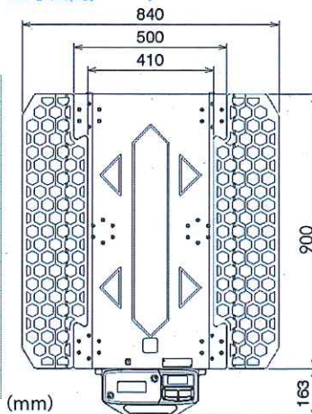
■寸法図(900mm)
